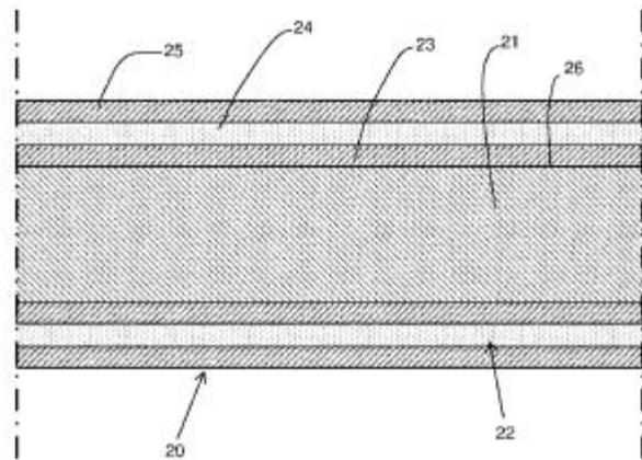
Figure 1 – Insulation System
